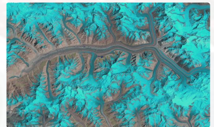
MOUNTAIN RANGE
