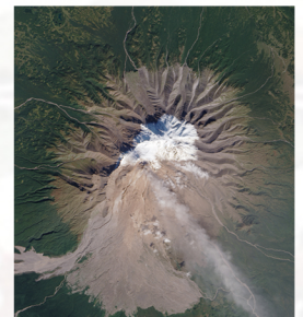
VOLCANO
