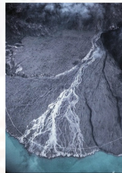
RIVER DELTA
